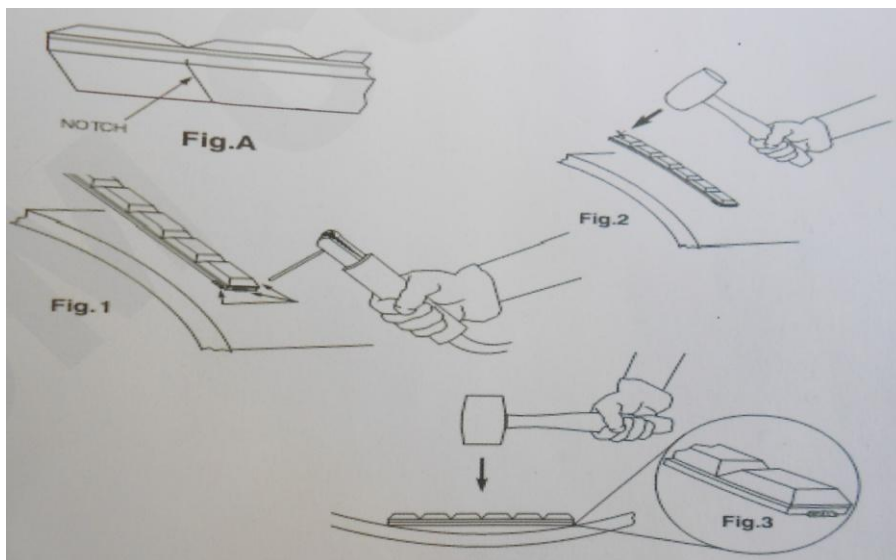
Picture 6-2 weldability wear-resistant bar/liner instructions
